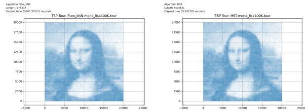
Figure 2: Visual comparison of Flow_kNN and MST tours.
